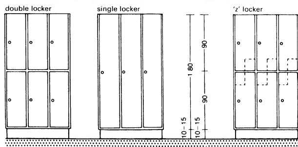
⑧ Clothes lockers
